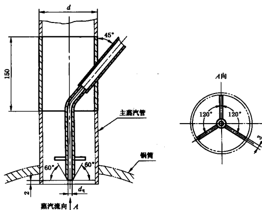
图 C.1 饱和蒸汽取样头
