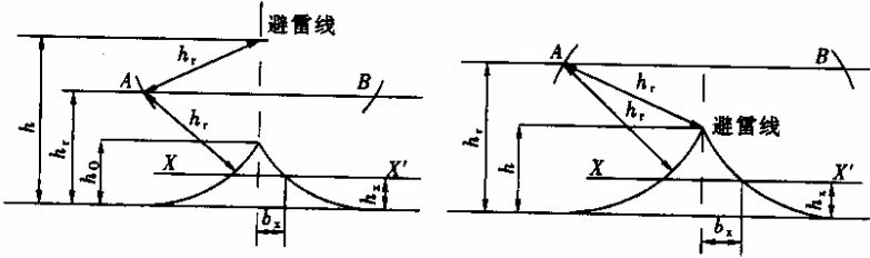
(a) h_r < h < 2h_r 时; (b) h \leq h_r 时
